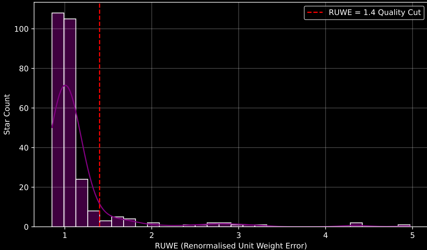
GALAH DR4 Field [6887] RUWE Distribution (n= 271)
