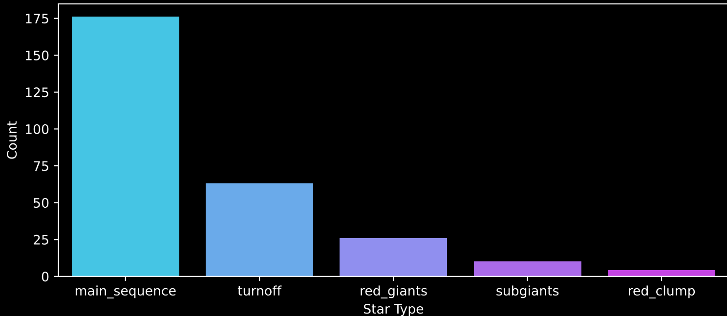
GALAH DR4 Field: [6887] Count plot of Star Type
